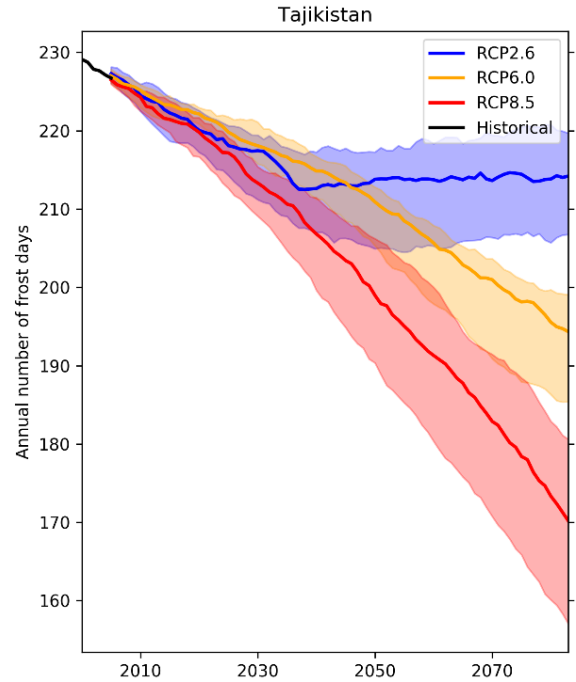
Figure 10: Number of frost days change projections for different GHG emissions scenarios (colour) and historical values (black). Each coloured line represents the 30-year running mean of the model ensemble under a given emissions scenario. Shaded areas represent the range of the model ensemble.
